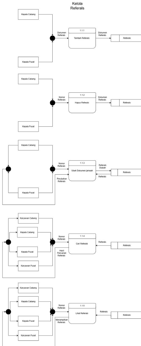
Gambar 4.33 Data Flow Diagram Referrals
