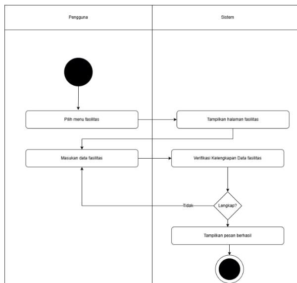
Gambar 4.22 Activity Diagram Tambah Fasilitas
