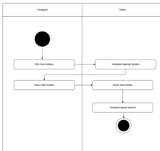
Gambar 4.24 Activity Diagram Hapus Fasilitas
