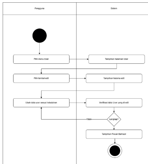
Gambar 4.3 Activity Diagram Ubah User
