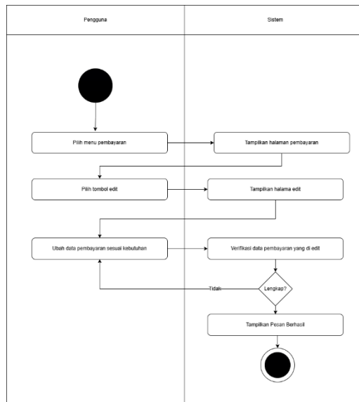
Gambar 4.11 Activity Diagram Ubah Pembayaran
