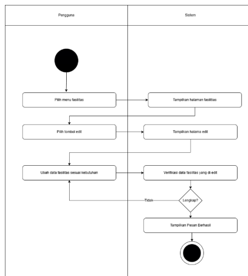
Gambar 4.23 Activity Diagram Ubah Fasilitas
