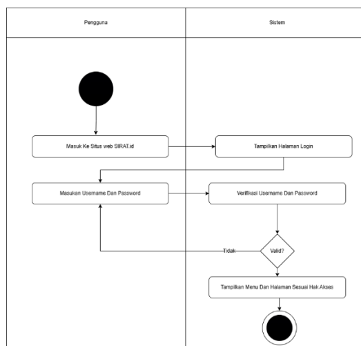
Gambar 4.1 Activity Diagram Login
