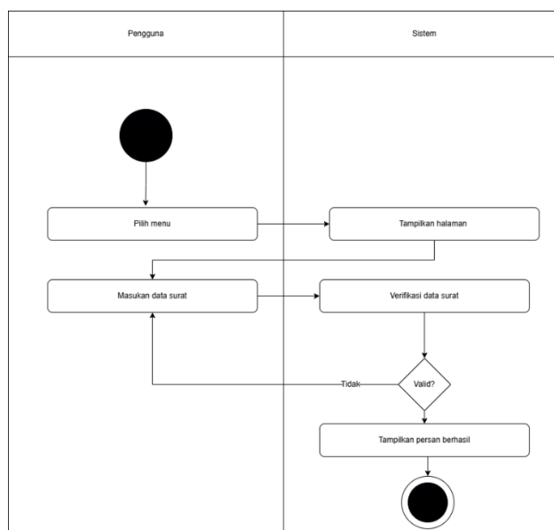
Gambar 4.6 Activity Diagram Tambah Surat
