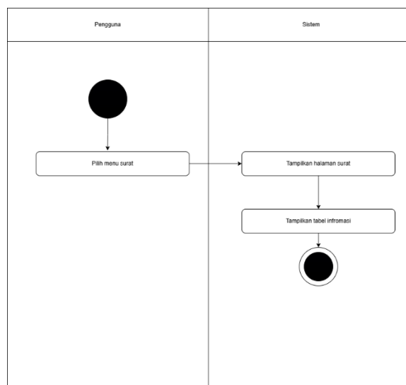
Gambar 4.9 Activity Diagram Lihat Surat
