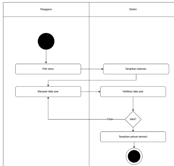
Gambar 4.2 Activity Diagram Tambah User
