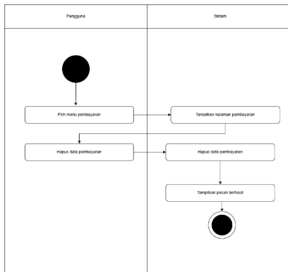
Gambar 4.12 Activity Diagram Hapus Pembayaran
