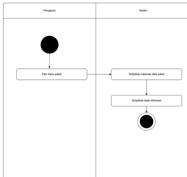
Gambar 4.17 Activity Diagram Melihat Paket
