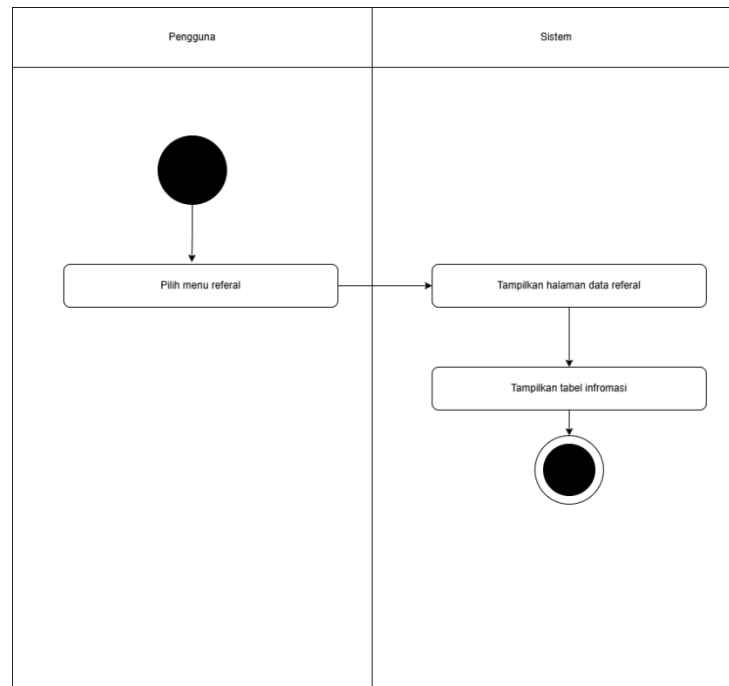
Gambar 4.26 Activity Diagram Lihat Referrals
