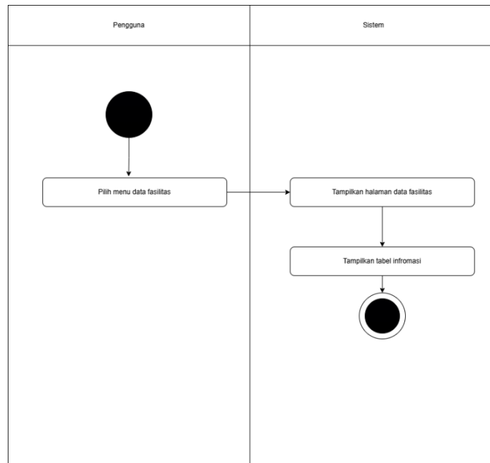
Gambar 4.25 Activity Diagram Lihat Fasilitas
