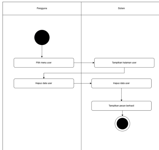
Gambar 4.4 Activity Diagram Hapus User
