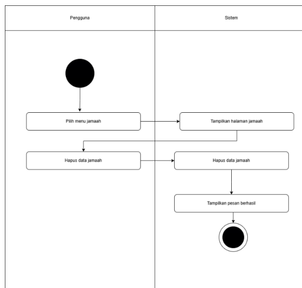
Gambar 4.20 Activity Diagram Hapus Jamaah
